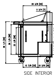
SIDE INTERIOR
