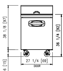
FRONT NLSMP27-12
