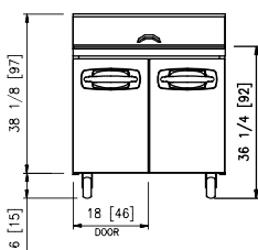
FRONT NLSMP36-15
