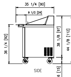
SIDE VIEWS ALL MODELS
