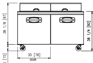
FRONT NLSMP60-24
