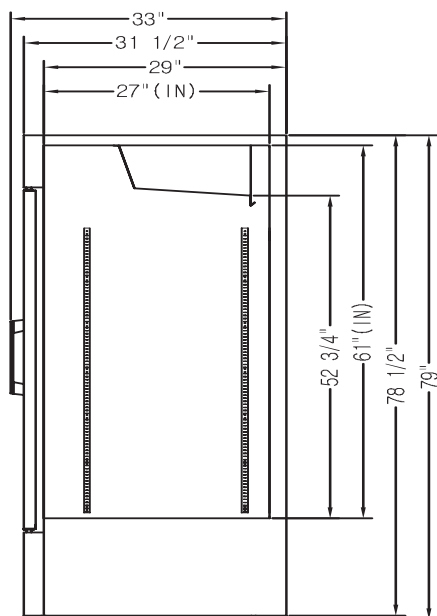
SIDE VIEW NLGR70H-B
