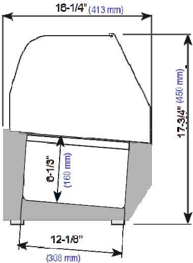
RIGHT VIEW
