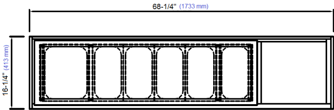
PLAN VIEW
