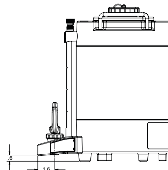
1.5 Gal TF Mechanical Baseless Server
