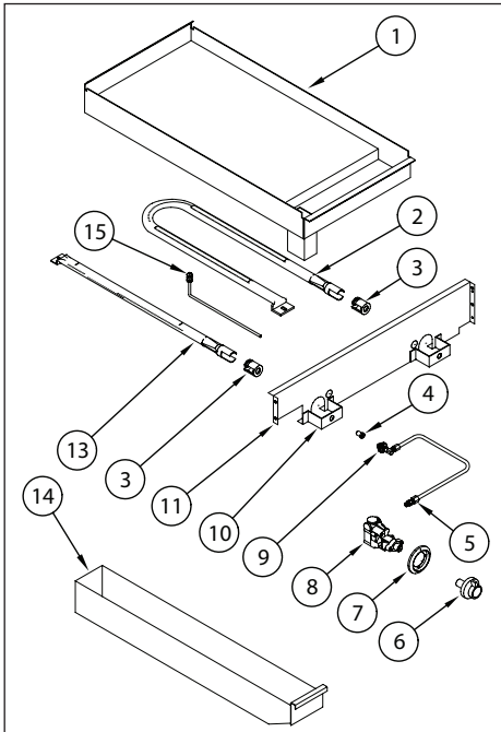
THERMO GRIDDLE
